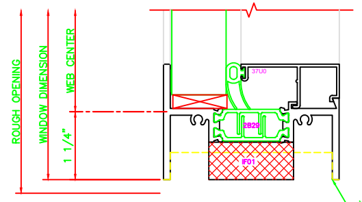
200 SILL 325 FIXED
